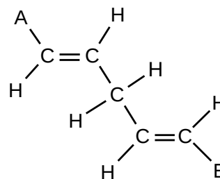
trans,trans-isomer
