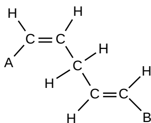
cis,trans-isomer
