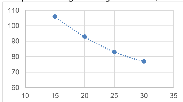
Graph of bending stress against P for Q = 170
