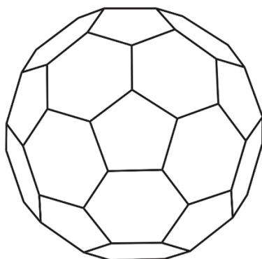
buckminsterfullerene, C_{60}
